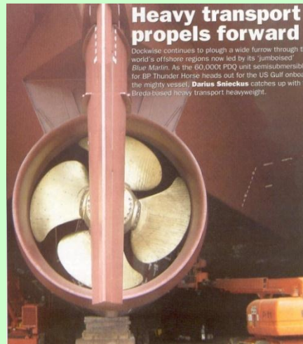
Ducted
